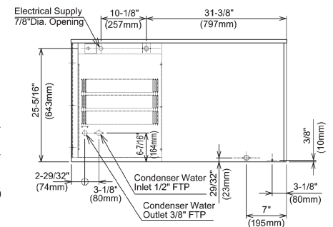
WATER-COOLED UNIT
