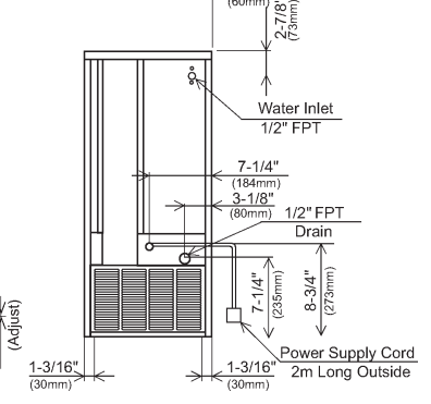
BACK DIMENSIONS (ADA compliant unit)
