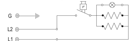
Wiring diagram
